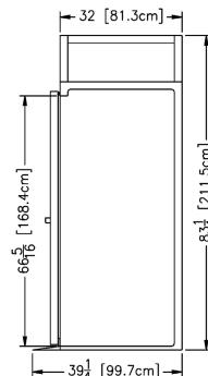
Section - RET232LUT-FHS
