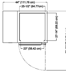
Plan - TU044HT
